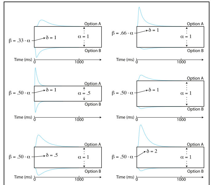
Figure 2. An illustration of how changing diffusion model parameters impacts decisions and response time distributions (in blue). We assume that evidence is correctly accumulated toward Option A. Top panel: higher relative start point \beta increases the likelihood and speed of selecting Option A by primarily increasing modal response speed. Middle panel: higher threshold \alpha increases the likelihood of choosing Option A and decreases the speed of choosing both options by shifting the mode and lengthening the tails of responses. Bottom panel: higher drift rate \delta increases the likelihood and speed of selecting Option A by shortening the tails of the responses. Nondecision time \tau is not depicted as it simply shifts both distributions by a fixed amount.
